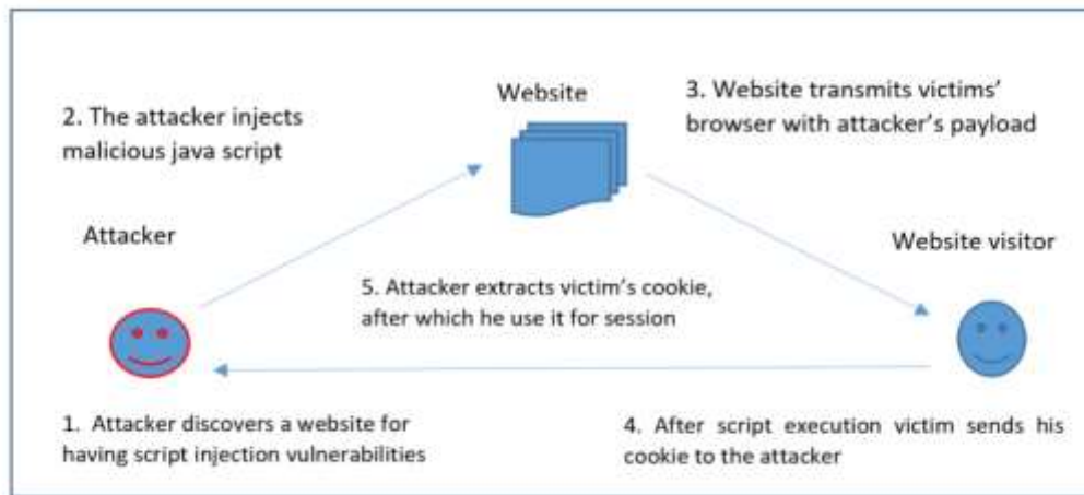
Figure 2: Scripting attack in website.
